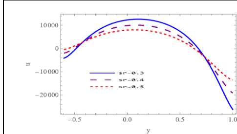
Figure 14- variation of u with respect to (Sr) values when Ha=3, A=5, \beta=0.1, Da=6, \Omega=0.3, w=0.3, \phi=0.5, kr=0.5, B=0.1, Gc=0.8, Gr=1.8, Sc=0.8, Sr=1.8 .
