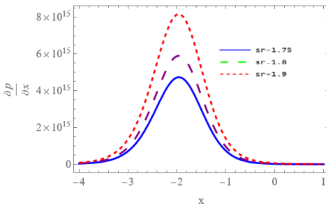
Figure 28- variation in \left(\frac{dp}{dx}\right) for various values of (Sr) when Ha=3, A=5, B=0.1, \beta=0.1, w=0.3, Da=6, kr=0.5, Gc=0.8, \Omega=0.3, \phi=0.5, Gr=1.8, Sc=1.8, Sr=1.8 .
