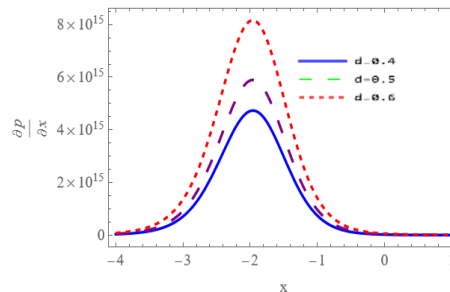
Figure 29 - variation in \left(\frac{dp}{dx}\right) for various values of (d) when Ha=3, A=5, \beta=0.1, Da=6, \Omega=0.3, w=0.3, \phi=0.5, kr=0.5, B=0.1, Gc=0.8, Gr=1.8, Sc=0.8, S=1.8 .
