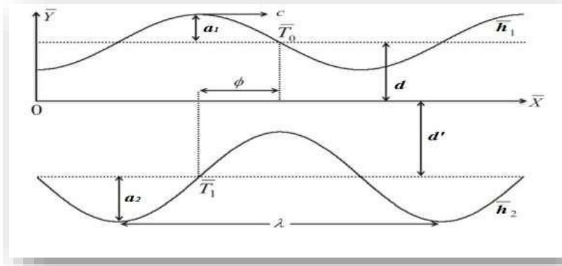
Figure 01- Channel coordinates in dimensional systems using cartesian asymmetry
