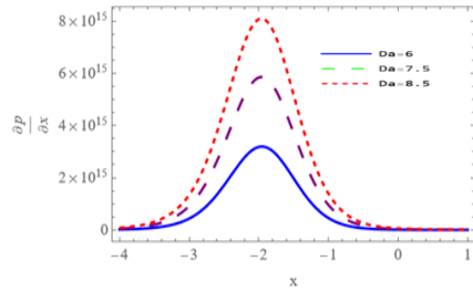
Figure18- variation in \left(\frac{dp}{dx}\right) for various values of (Da) when Ha=3 , \beta=0.1, \Omega=0.3, w=0.3, \phi=0.5 , A=5, B=0.1 kr=0.5, Gc=0.8, Gr=1.8, Sc=0.8, Sr=1.8 .
