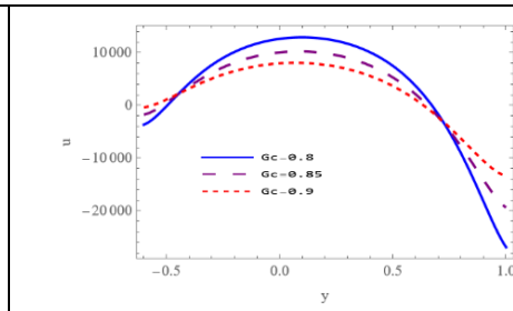
Figure 11- variation of u with respect to (Gc) values when Ha=3, A=5, \beta=0.1, Da=6, \Omega=0.3, w=0.3, \phi=0.5, kr=0.5, B=0.1, Gc=0.8, Gr=1.8, Sc=0.8, Sr=1.8 .
